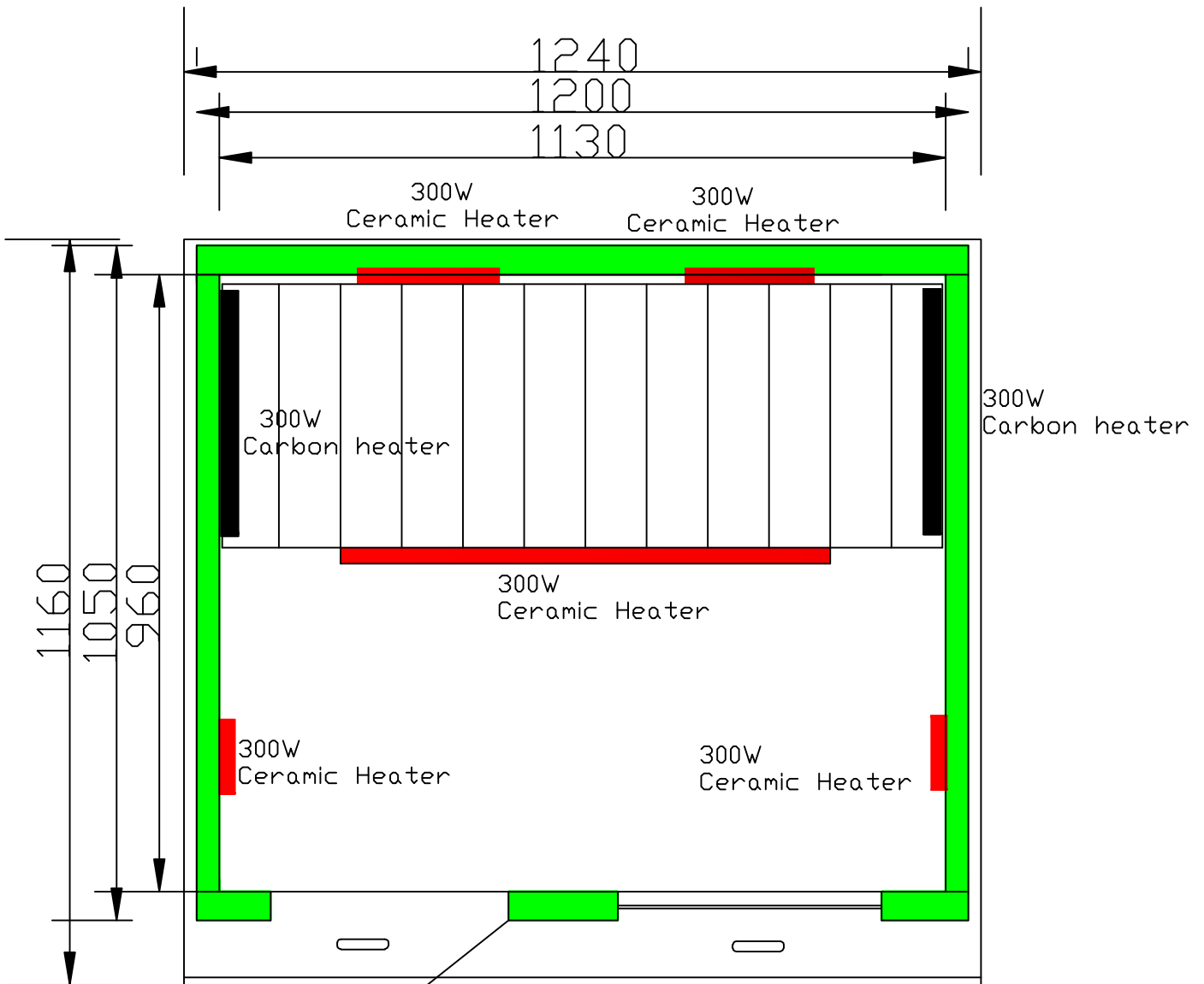
KD-5002SC Size:1200×1050×1900mm capacity:2person Power:2100W
